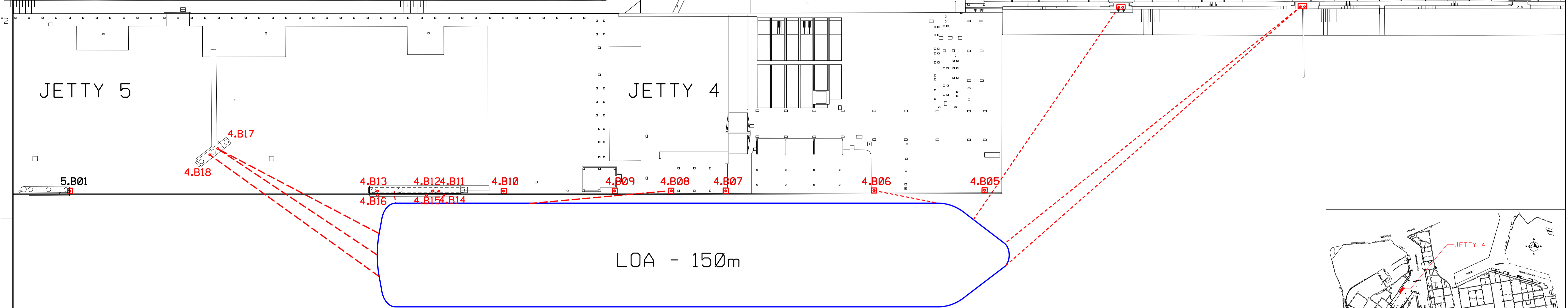
MOORING PLAN JETTY 4 10 - 25,000 SDWT VESSELS
